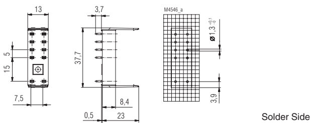
Solder Side
