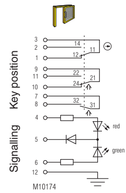
Fig. 2: Lock deactivated: 1st key inserted, 2nd key removed
