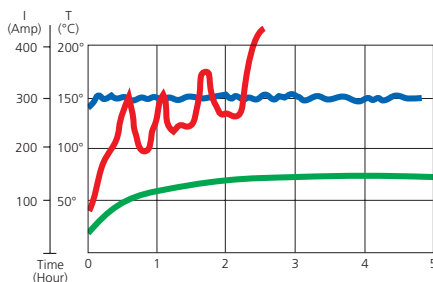
— Continuous current 300 Amp — Temperature Carbon brush — Temperature Kp-brush
