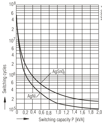
OA 5668: Contact service life (at t_u = 20^\circ\text{C} )
