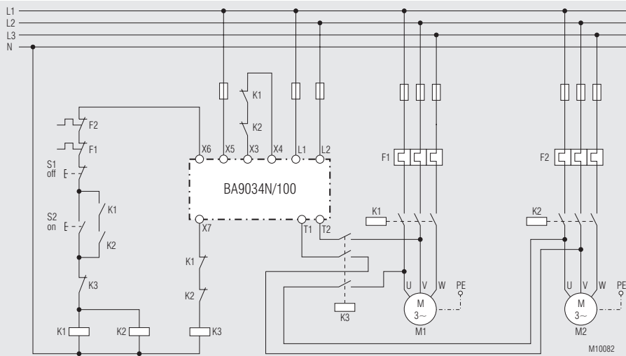
BA 9034N/100 simultaneous braking of 2 motors in serial connection
