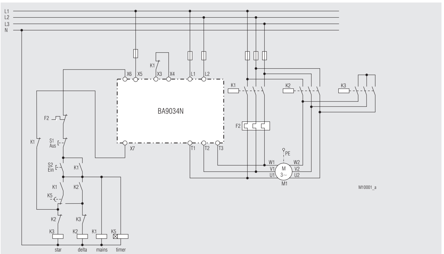
BA 9034N, 3-phase, \star - \Delta -start up
