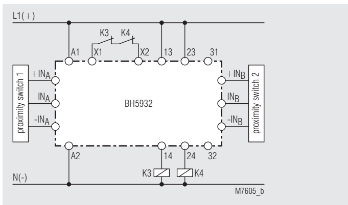
Connection with external contactors
