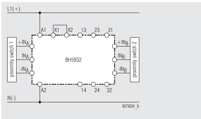
Standard connection
